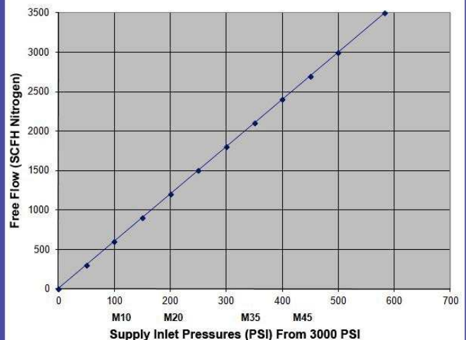
Servo-Max "M" Series Maximum Flows at Minimum Pressures
