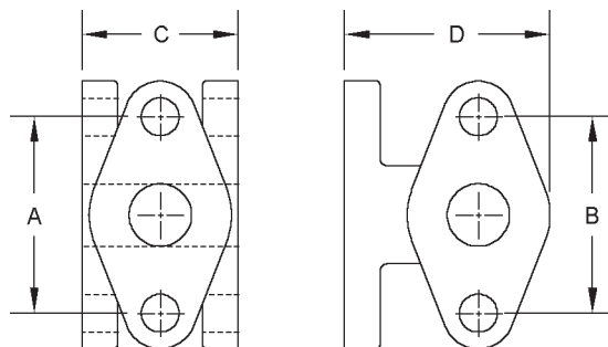
3/4" X 3/4" X 3/4" FLANGE FITTING TEE WITHOUT GASKET GROOVE
