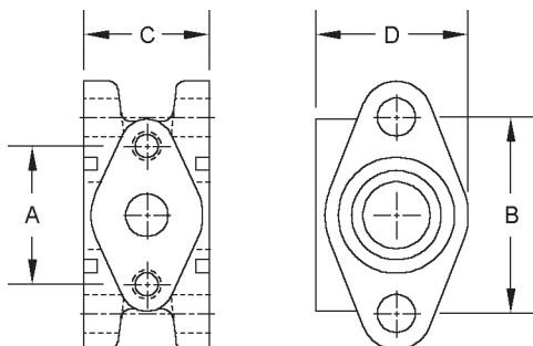
3/4" X 3/4" X 3/8" FLANGE FITTING TEE WITH GASKET GROOVE
