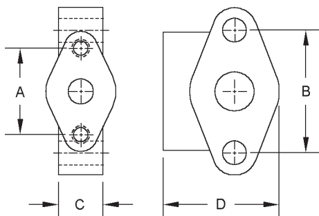
3/4" X 3/4" X 3/8" FLANGE FITTING TEE WITHOUT GASKET GROOVE
