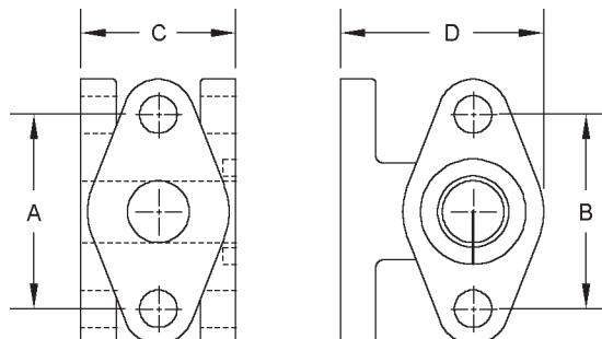
3/4" X 3/4" X 3/4" FLANGE FITTING TEE WITH GASKET GROOVE
