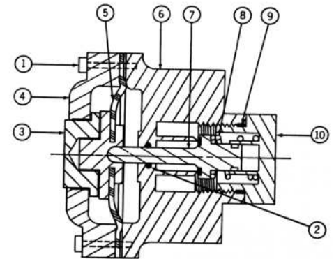
Shut-off Valve
