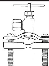
104SDHB Self Drilling Valve Assembly fits 3/8" thru 1-3/8" O.D. Copper Tubing with Heavy Bracket
