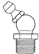
65° 1/8 Pipe Thread
