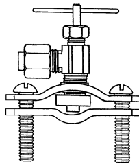
Valve With Brass Saddle
