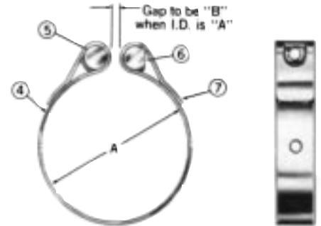
Band Assembly
