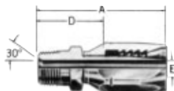
Male pipe 4729-S
