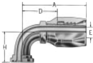
Code 61 SAE J518c 90° split flange (short) 479003-S
