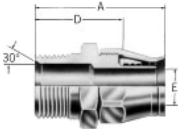
Male pipe 38-190627
