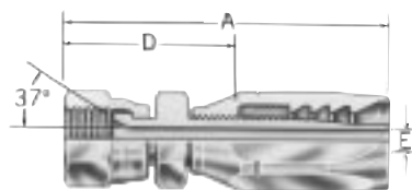
SAE 37° (JIC) swivel 4730-S
