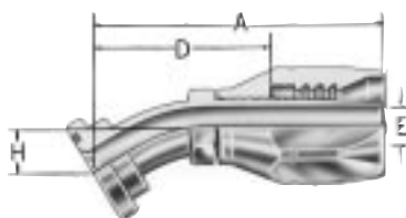
Code 61 SAE J518c 45° split flange 474503-S
