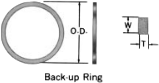
Back-up Ring 22006 (Commercial grade leather)
