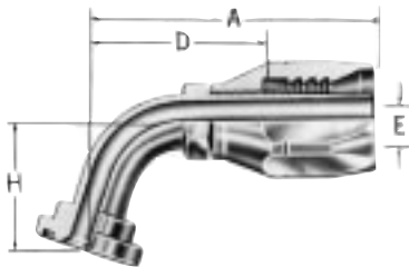
Code 61 SAE J518c 67½° split flange 476703-S
