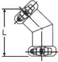
Basic part number: NH1617 NH1667 Allowable misalignment: \pm 2' per end
