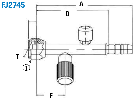
Straight Female O-ring (Long Pilot), R134a Hi-Side Port and Switch Port (Port to Port Rotations will vary - Contact Eaton Application Engineering)
