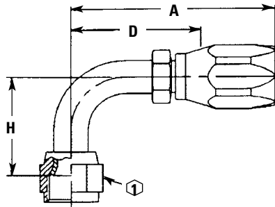
90° Elbow 190295 Universal Swivel (Long Drop), 190301 S.A.E. 45° Swivel 190260 S.A.E. 37° Swivel
