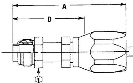
Male O-ring Pilot (Short)
