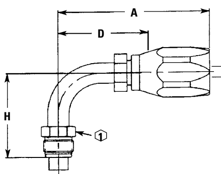
90° Male O-ring Pilot (Short)
