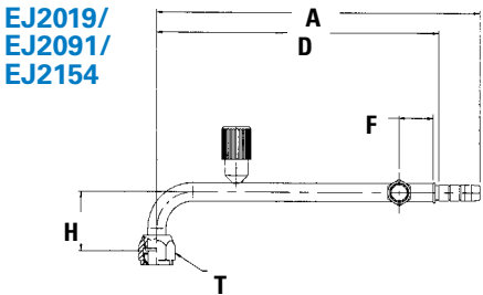
90° Female O-ring (Long Pilot), R134a Hi-Side Port and Switch port (Port to Port Rotations will vary - Contact Eaton Application Engineering)
