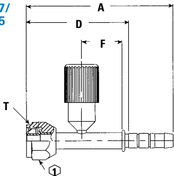
Female O-ring (Long Pilot) with High Side Charge Port
