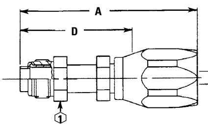
Male O-ring Pilot (Long)
